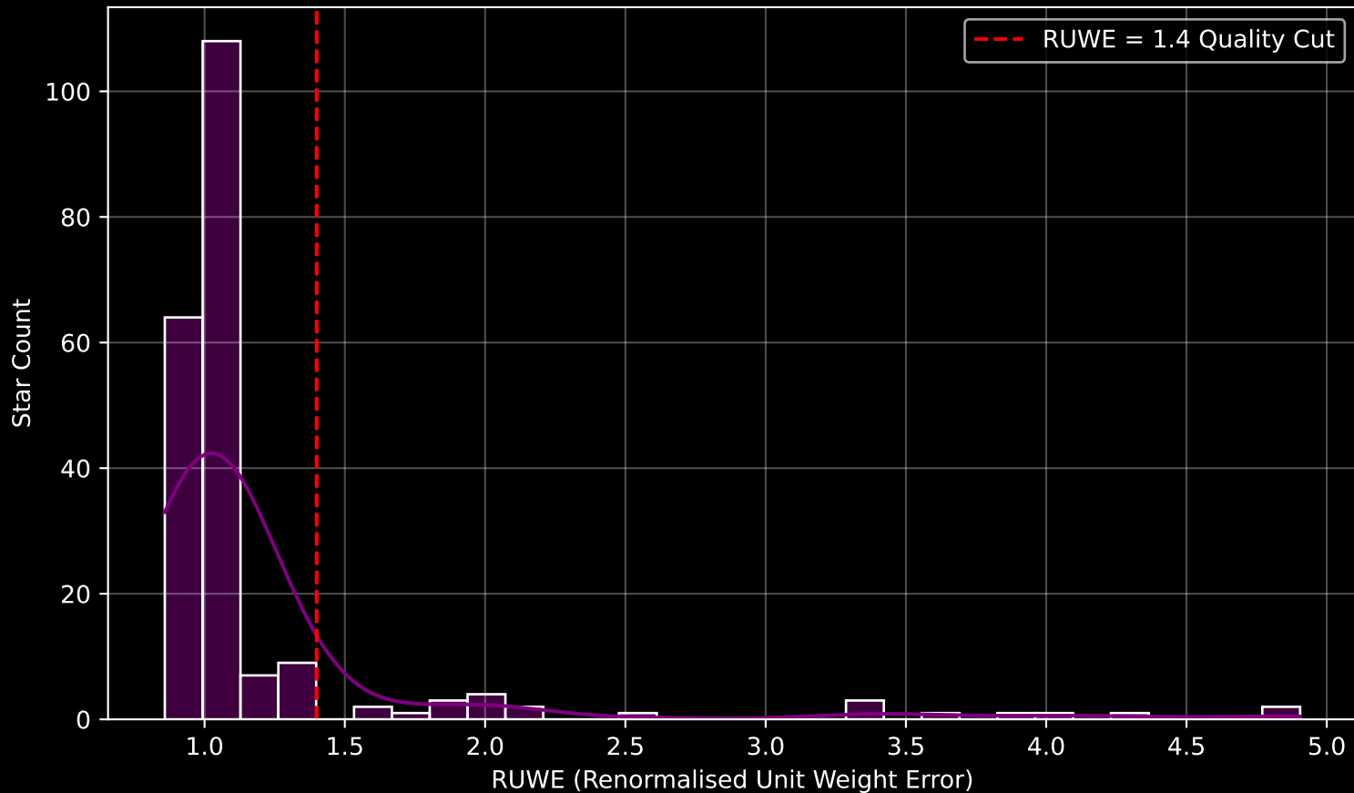
GALAH DR4 Field [9468] RUWE Distribution (n= 210)
