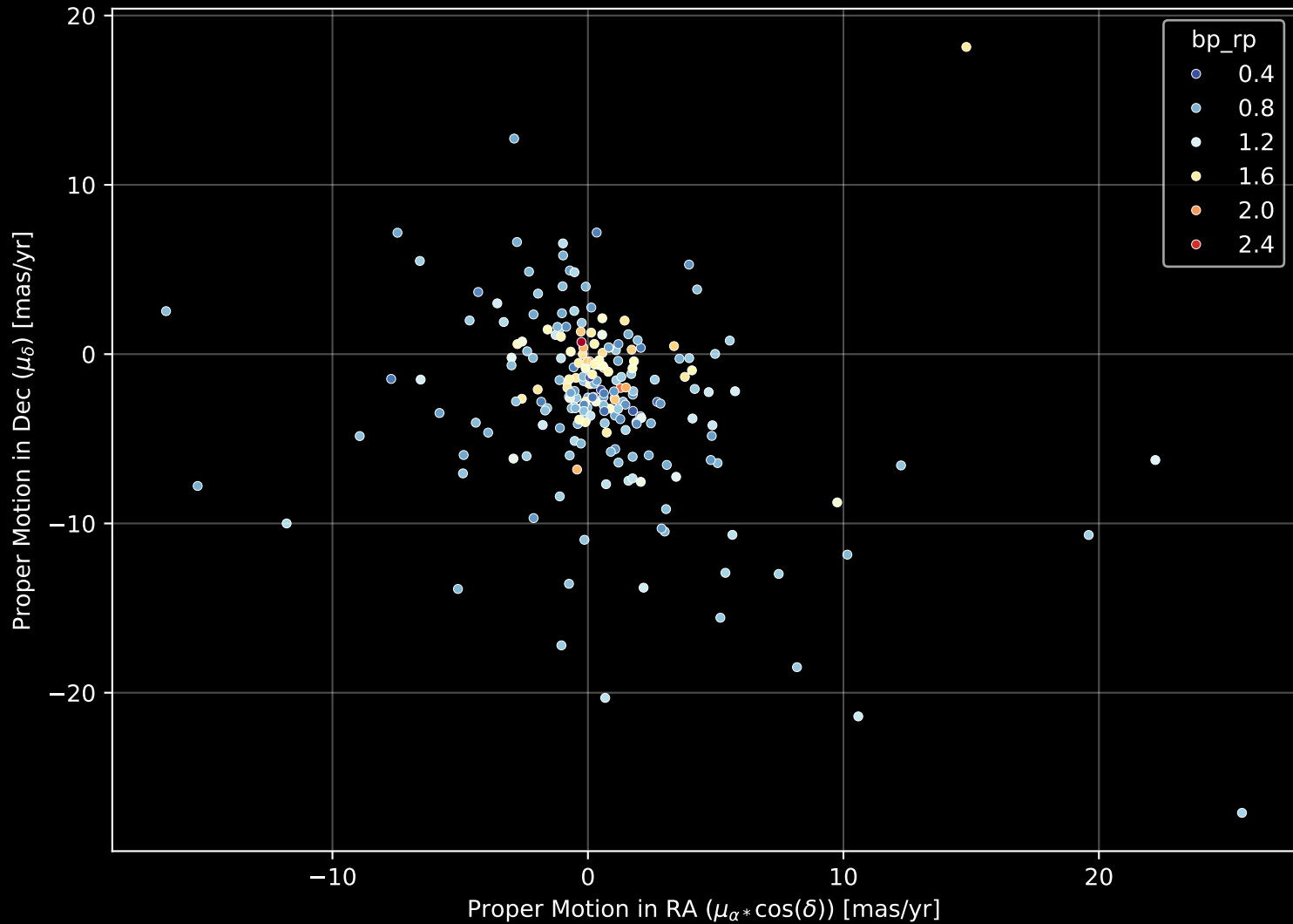
GALAH DR4 Field: [9468] Proper Motion Diagram (n= 215)
