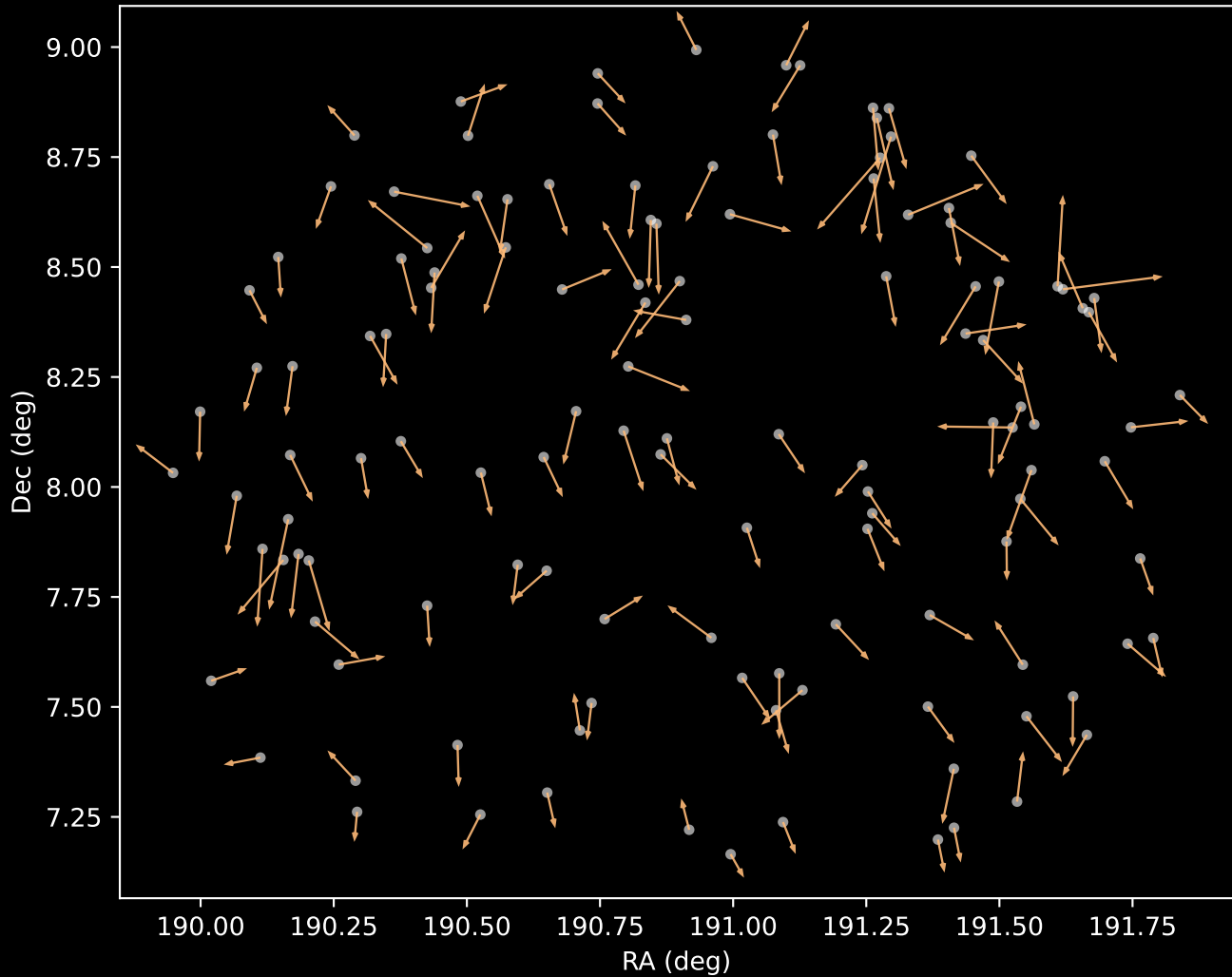
GALAH DR4 Cluster 3 Proper Motion Vectors (n=126)
