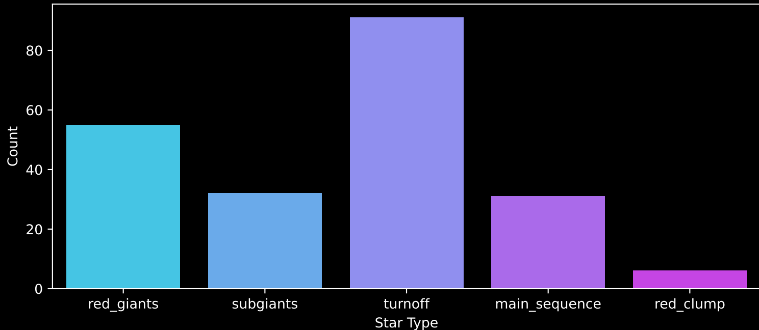
GALAH DR4 Field: [9468] Count plot of Star Type
